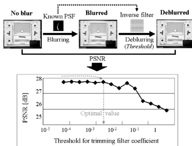
Fig. 2 Relationship between PSNR and threshold for trimming filter coefficients.
