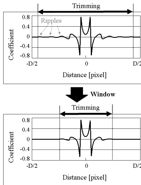
Fig. 3 Example of window function.
