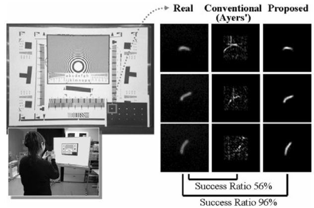
Fig. 5 Experiment of PSF estimation.
