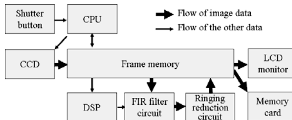
Fig. 9 Block diagram of hand-blur refiner.
